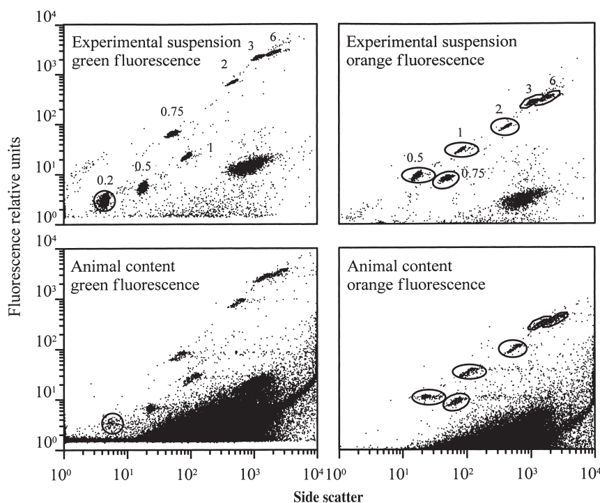
Fig. 1. Example of flowcytometer plots representing side scatter (directly related to particle size) versus green- and orange-fluorescence. Upper panels: microspheres in the experimental suspension; lower panels: microspheres in appendicularian guts. Green fluorescence was used to discriminate 0.2 \mu\text{m} microspheres, while orange fluorescence was used for 0.5, 0.75, 1, 2, 3 and 6 \mu\text{m} microspheres. Oval shapes delimit the boundaries used to discriminate the number of each bead size. Axis units are relative. The thick, small, densely packed cluster of points in the lower part of the upper panels, and the thick and much larger cluster of points in the lower part of the lower panels correspond to Tetraselmis sp. cells before and after being ground with a tissue grinder, respectively. Note that there is nearly no overlap between these clusters of points and the ones corresponding to microbeads
