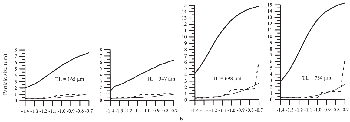
Fig. 5. Oikopleura dioica . Variation of P_{90} (thick continuous line) and P_{10} (thin continuous line; these 2 parameters define a particle size range that encloses 80% of the diet, see methods), and P^* (dashed line; particle size with the highest contribution to the diet) versus the exponent of the biomass spectrum, b (see 'Materials and methods' for calculation of these parameters). Each panel corresponds to each of the 4 retention efficiency experiments performed on O. dioica , indicated by their average trunk length (TL)
