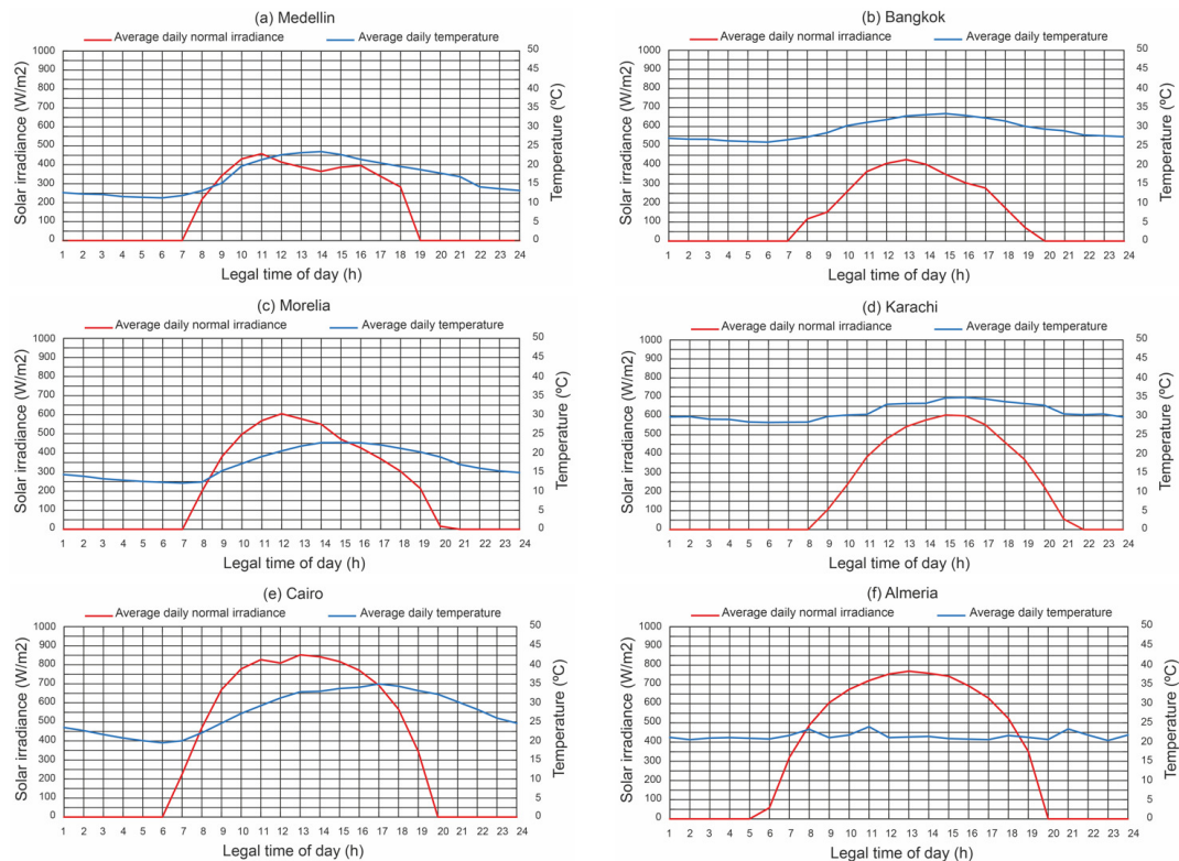
Figure 11. Environmental conditions.
