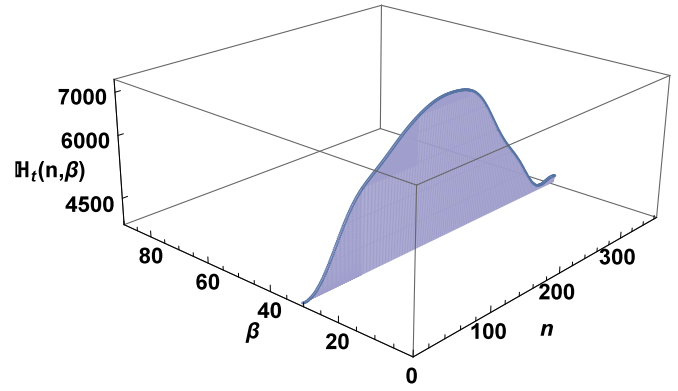
Fig. 7. Annual irradiation for \beta_{opt}^y .
