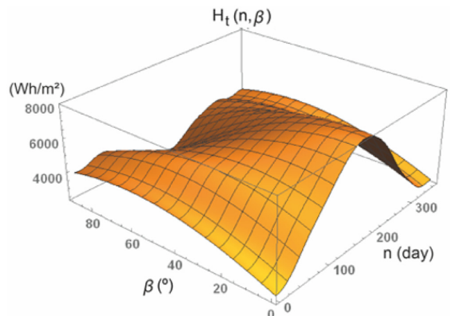
Fig. 1. Total daily solar irradiation on a tilted surface H_t(n, \beta) .
