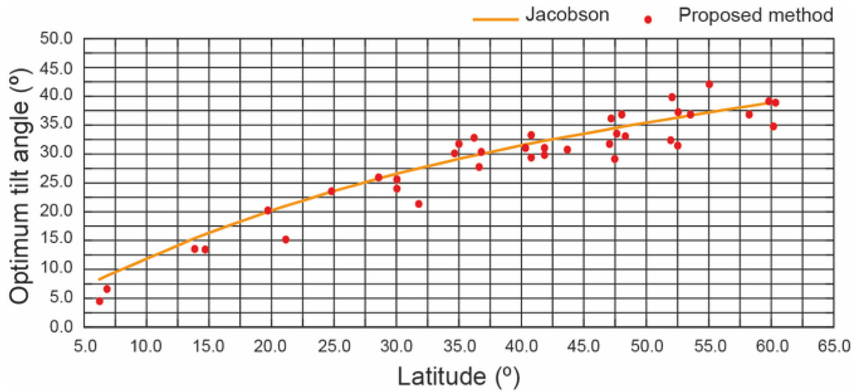
Fig. 8. Optimum tilt angle for cities under study and Jacobson's formula.
