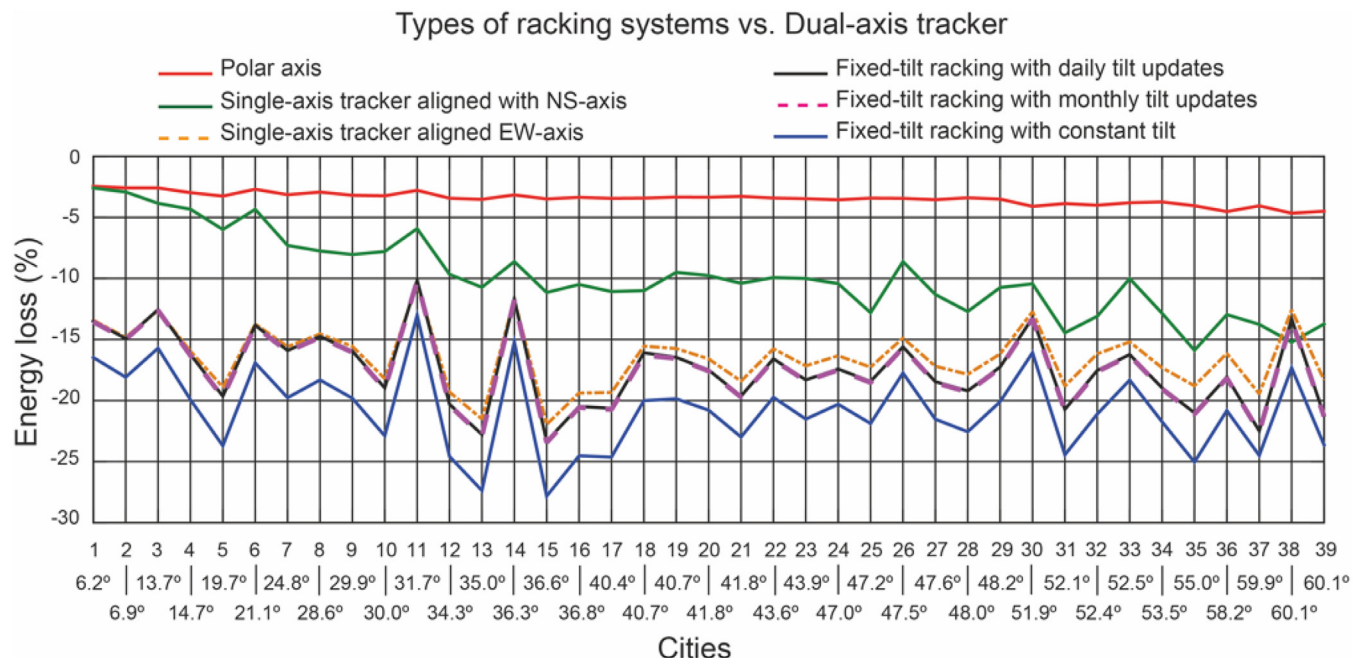
Fig. 10. Ratio of energy loss with respect to the dual-axis tracker. Notice that the daily and monthly plots overlap.
