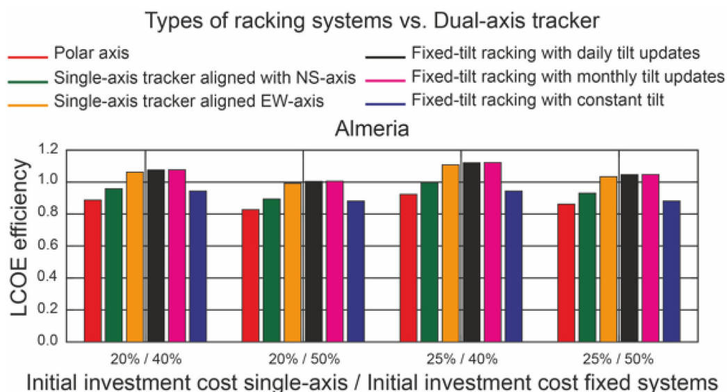
Fig. 14. Sensitivity analysis of LCOE with respect to the dual-axis tracker in Almeria.
