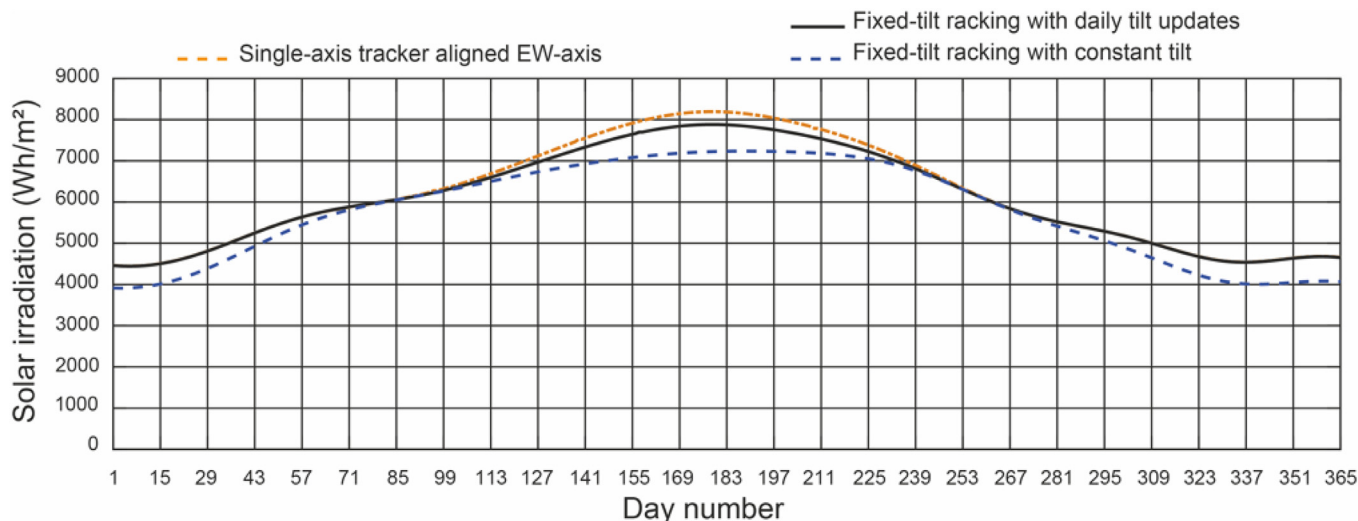
Fig. 12. Daily irradiation in Almeria (nr. 16).
