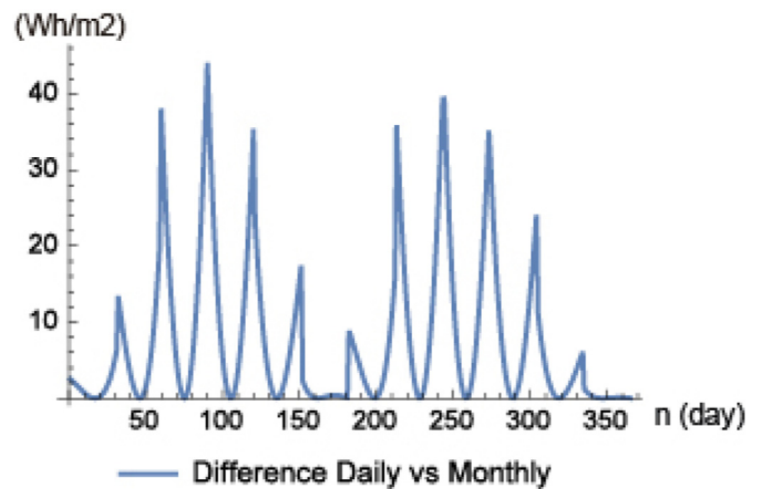
Fig. 11. Difference in irradiation between daily and monthly tilt updates.
