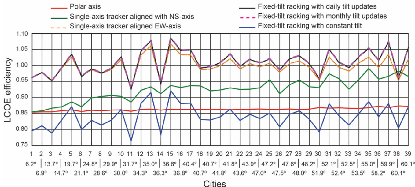
Fig. 13. LCOE efficiency with respect to the dual-axis tracker. Notice that the daily and monthly plots overlap.
