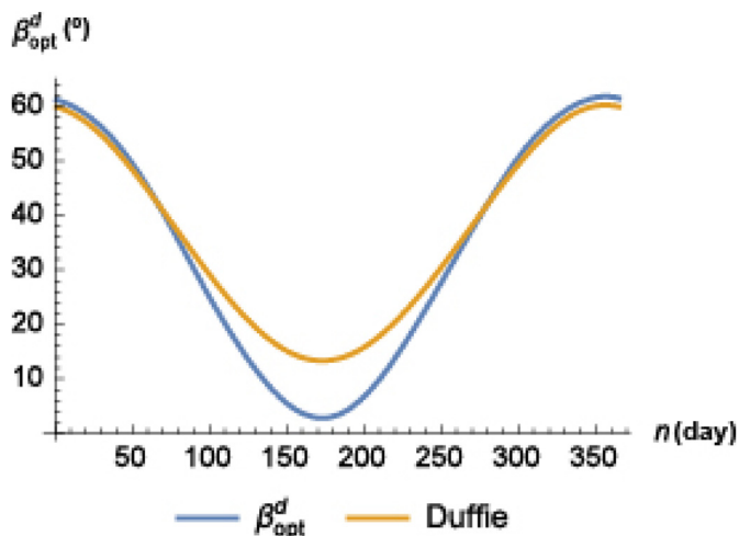
Fig. 5. Daily values of \beta_{opt}^d(n) and Duffie's formula (6).
