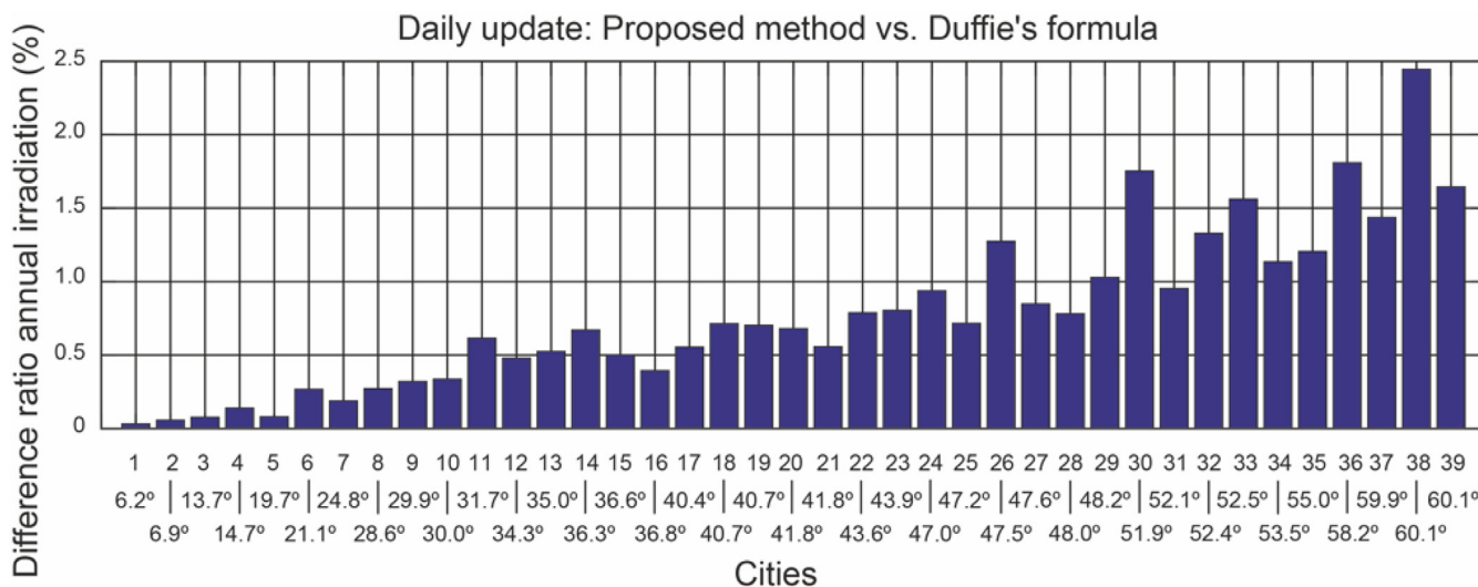
Fig. 4. Difference ratio of total annual irradiation between proposed daily update and Duffie's formula.
