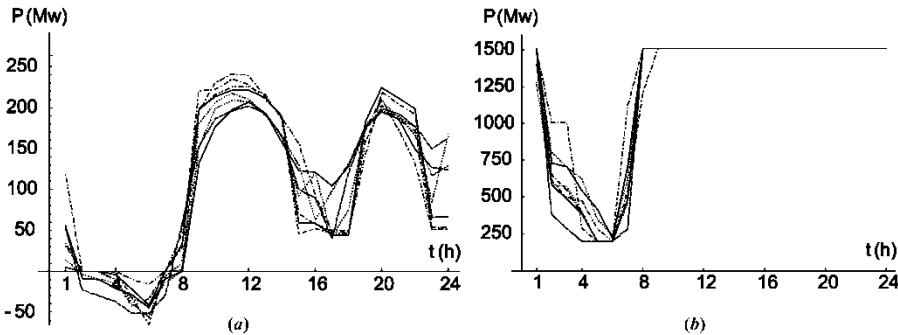
Figure 1. (a) Optimal hydro-power. (b) Optimal thermal-power.
