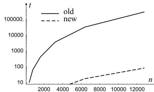
Fig. 1. CPU time.
