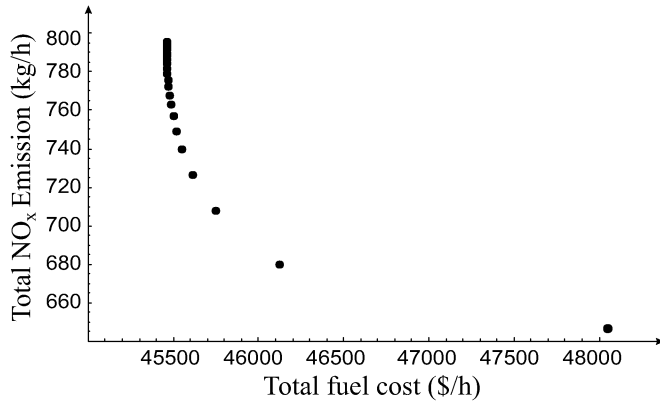
Fig. 3. Pareto-optimal front.
