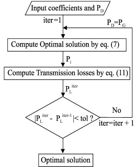
Fig. 1. Computational flow of the proposed iterative method.
