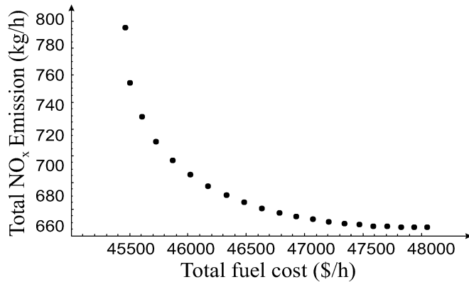
Fig. 4. Pareto-optimal front.
