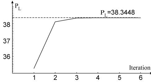
Fig. 2. Convergence of the iterative method.
