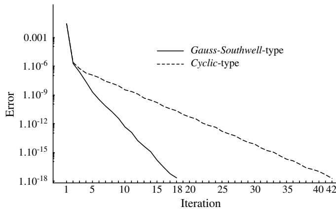
Fig. 4. Convergence with 20 hydro-plants.
