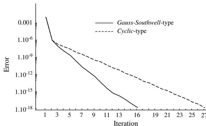
Fig. 3. Convergence with 10 hydro-plants.
