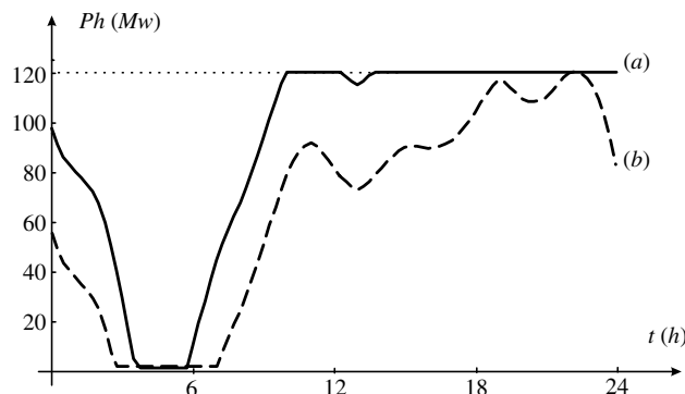
Fig. 1. Optimal hydro-power P_h(t) .
