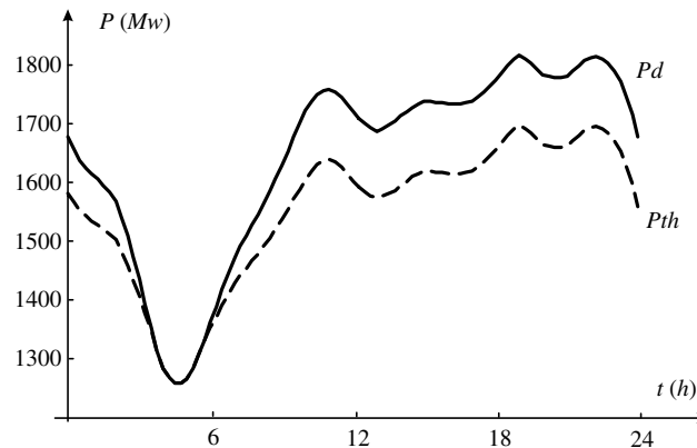
Fig. 2. Optimal thermal power P_{th}(t) and P_d(t) .
