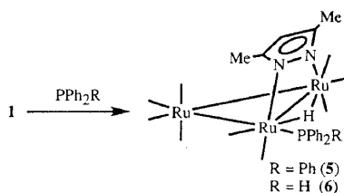
Scheme 3.
