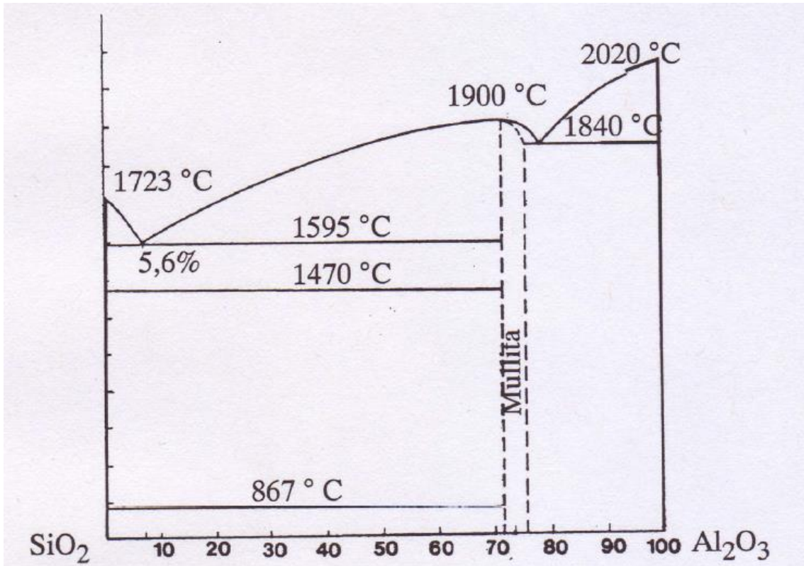
Fig. IX.48. Diagrama \text{SiO}_2 - \text{Al}_2\text{O}_3 .
